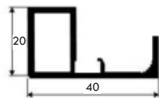
ZS-WP-02 Profile Handle (Left/Right) Size : 120mm/200mm
