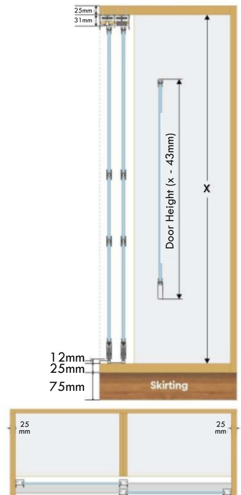
ZS-WP-123 Sliding Fitting for 2 Door Both Side Sliding Weight Capacity : 60 Kg.
