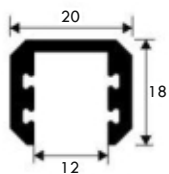
ZS-SP-01 BM Frame Profile
