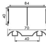
ZS-WP-103 Top/Bottom Profile
