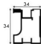
ZS-WP-105 Handle Profile - C
