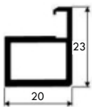
ZS-WP-01 Profile For Sutter
